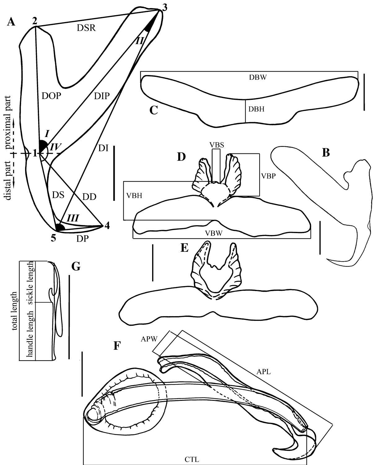
Fig. 1 The haptoral and copulatory hard-parts of Ligophorus bykhowskyi n. sp. from Crenimugil crenilabris in the Red Sea, showing the linear measurements and angles made for this and other Ligophorus spp. A, dorsal anchor; B, ventral anchor; C, dorsal bar; D, ventral bar (ventral view); E, ventral bar (dorsal view); F, male copulatory organ; G, marginal hook; I–IV angles. Abbreviations: See ‘Materials and methods’. Scale-bars: 10 \mu m
